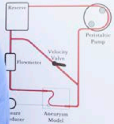
The physical cerebral aneurysm model was designed to facilitate according to general hemodynamic flow that have been shown to be linked to increased risk of rupture. Such as an elongated dome, dome parent/daughter angle, greater side/parent angle [1].
